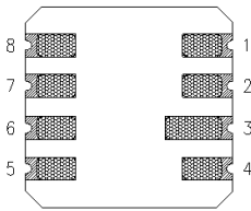
VERSION WITH CERAMIC CARRIER AND METAL CAP
